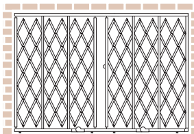
Pair Gate: Fixed Top & Fold-Away Bottom Track Max Width 32' | Max Height 12'
