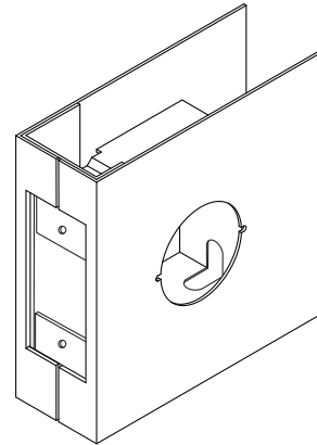
GOV'T G2 CYLINDRICAL LOCK
