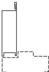
C.C.W. 48 C.C.W. 49 Recessed Sill
