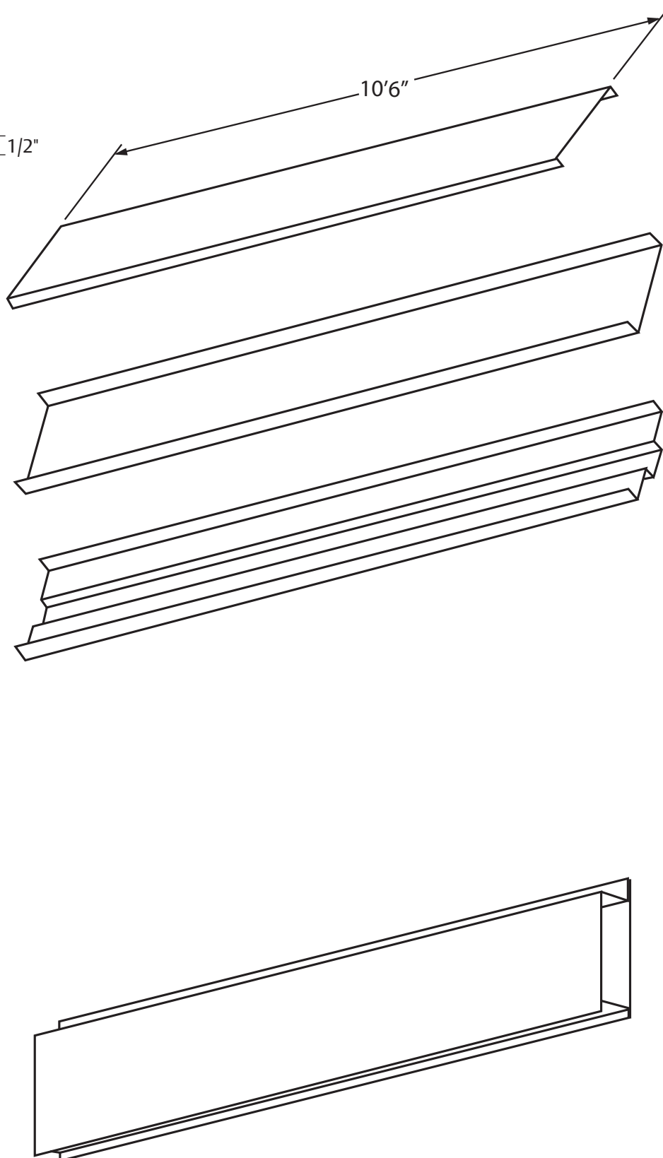
C.C.W. 28, 4" face Full Jamb Depth C.C.W. 139, 6" face Full Jamb Depth C.C.W. 140, 8" face - 10' max. Full Jamb Depth C.C.W. 55, 6-13/16" face Full Jamb Depth Sills
