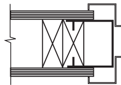
2 X 4 WOOD STUD WITH 5/8" SHEETROCK
